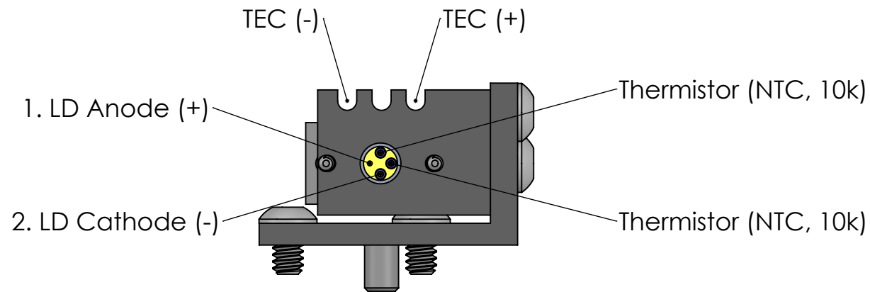
BACK VIEW
